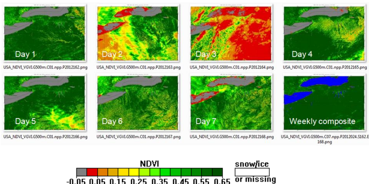
Figure 3.3-3 VIIRS NDVI from daily maps and seven days composite map.
